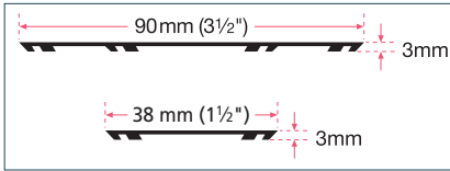
FIG. H - UV-resistant EPDM rubber joint sealing strip with ribs (supplied by AFC)
