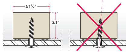
FIG. B-2 Interior Profile
