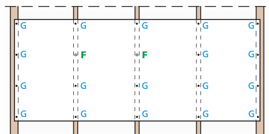
FIG. F - Horizontal installation on vertical profiles
