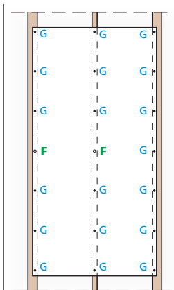
FIG. E - Vertical installation on vertical profiles
