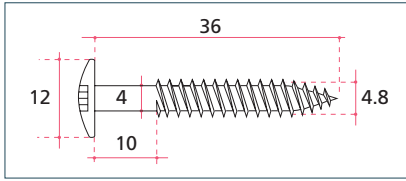
FIG. G - Screw (supplied by AFC)
