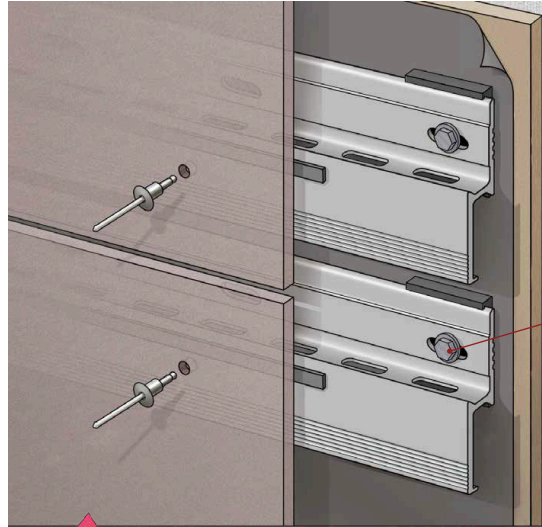
FIG. D-1B- Building wrap per AFC. Weather and UV resistant. Check local codes for proper placement.
