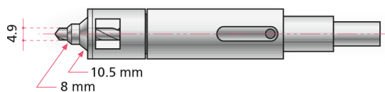
FIG. I Centralizing drill bit
